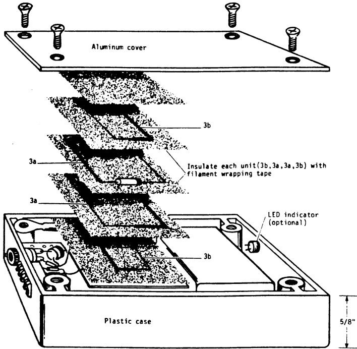
Figure 2 Parts Layout
