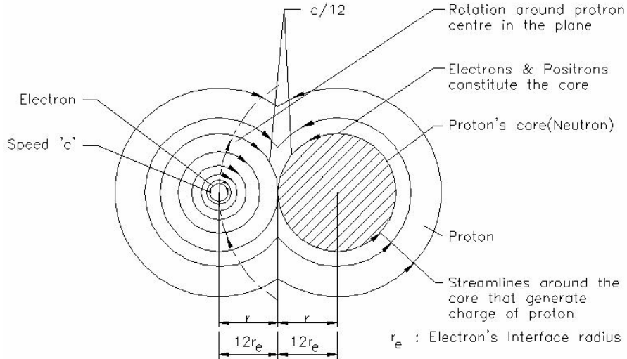
Fig. 11 Hydrogen Atom
