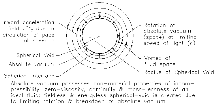
Fig. 2 Vortex in electron structure
