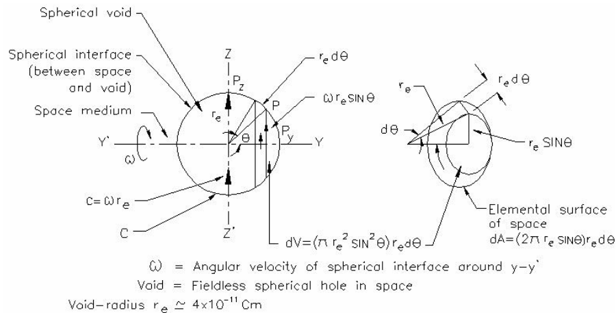
Fig. 3 Velocity Field on Interface
