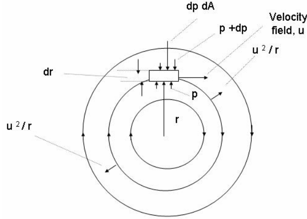
Fig. 1 Irrotational vortex
