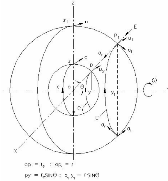
Fig. 5 Electric Field of Electron
