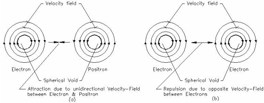
Fig. 4 Attractive &amp; Repulsive Forces due to Velocity Fields
