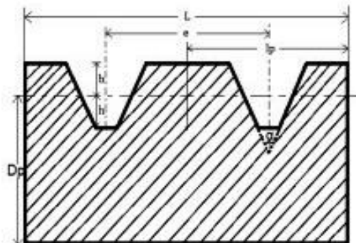
Fig :- V-Belt Pulley Detail
