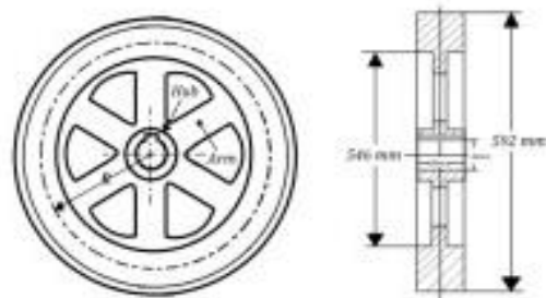
Fig - Flywheel
