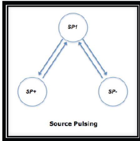
Fig. 10 - The self-generated fission-fusion process of SP1 or Partiki
