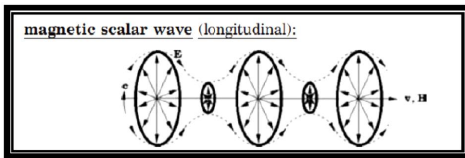
Fig. 12 - Electric ring vortices form a magnetic wave.
