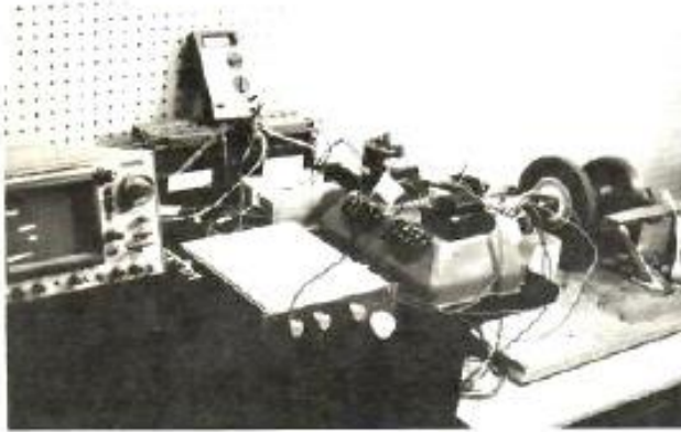
Figure 3. 1st Prototype, Total system
