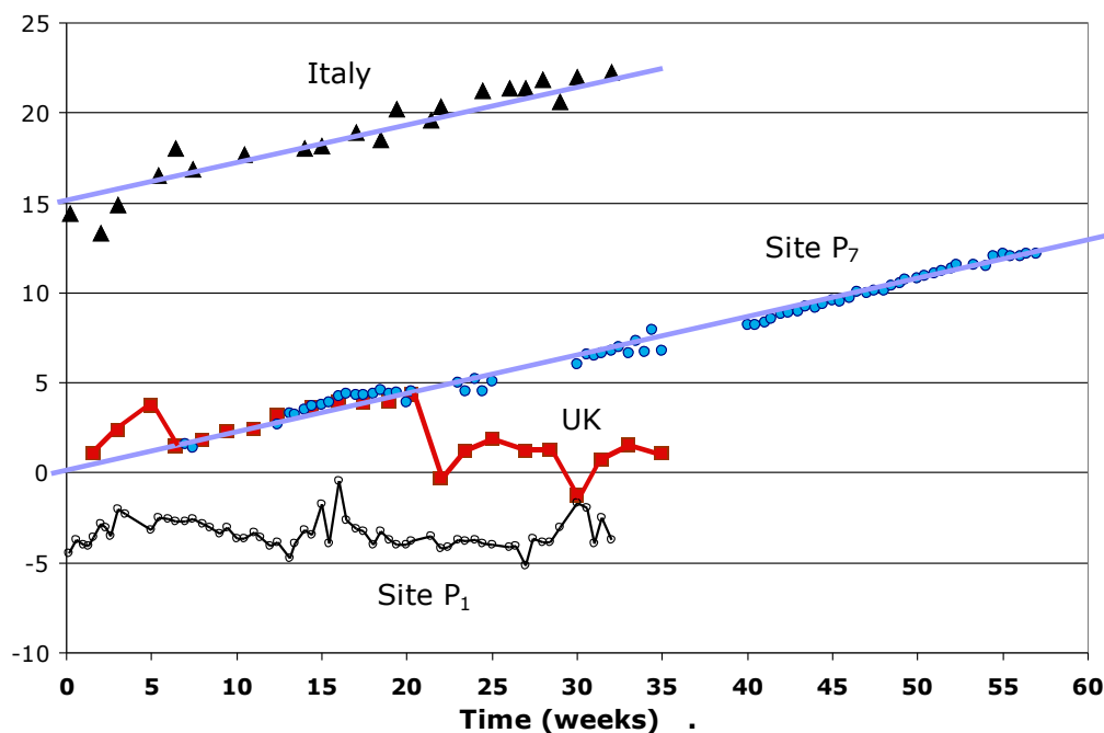
Figure 6. \delta G_{\text{H}^+}^* vs. time at four diverse sites.
